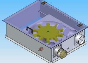
Umlenk-/Spannstation
